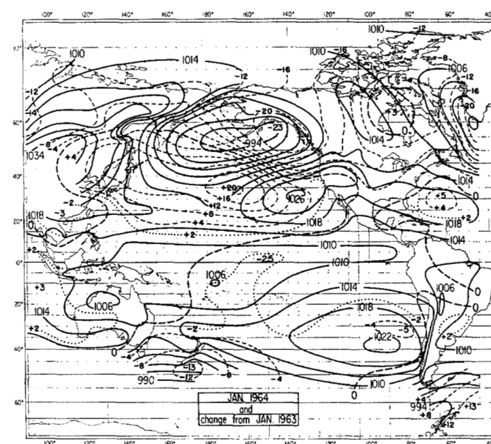
FIGURE 3.—January 1964 distribution of pressure (millibars) at sea level. Change from January 1963 in dashed isallobars.
